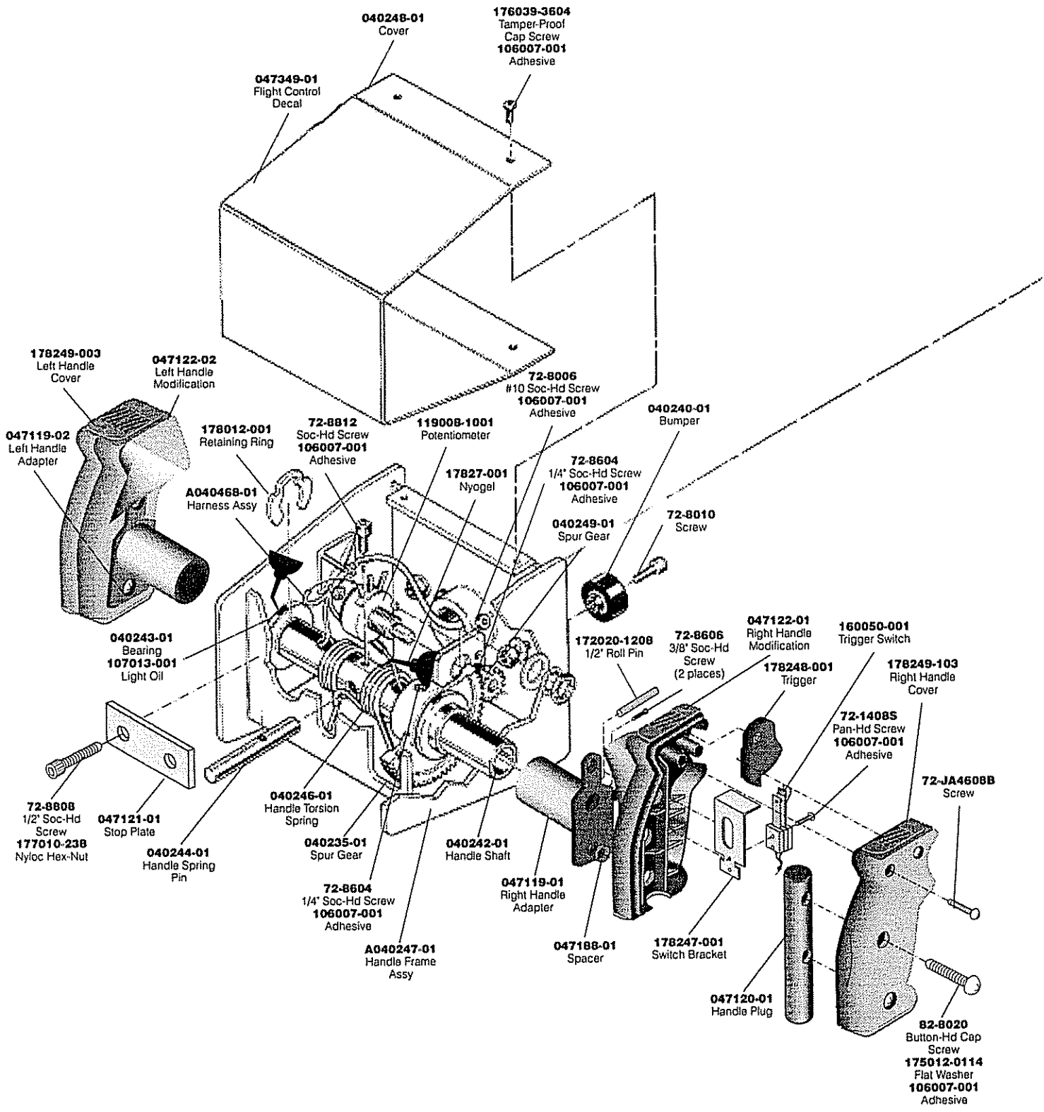
Figure 4-2 Flight Control Assembly A042562-02 B
